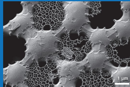
The delicate open structure of a non-conductive diatom can be imaged at low kV in high vacuum without charging artefacts with the ETSE.
